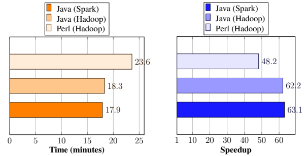
Fig. 2: Performance of the PoS Tagger considering different Big Data engines when processing the complete Wikipedia on a cluster: execution time (left) and speedup (right).
