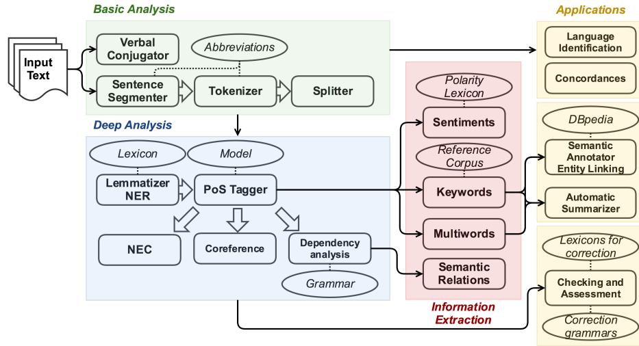
Fig. 1: Architecture of LinguaKit.
